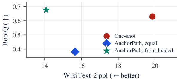
(b) ppl \leftrightarrow BoolQ front ( \rho = 0.3 )
